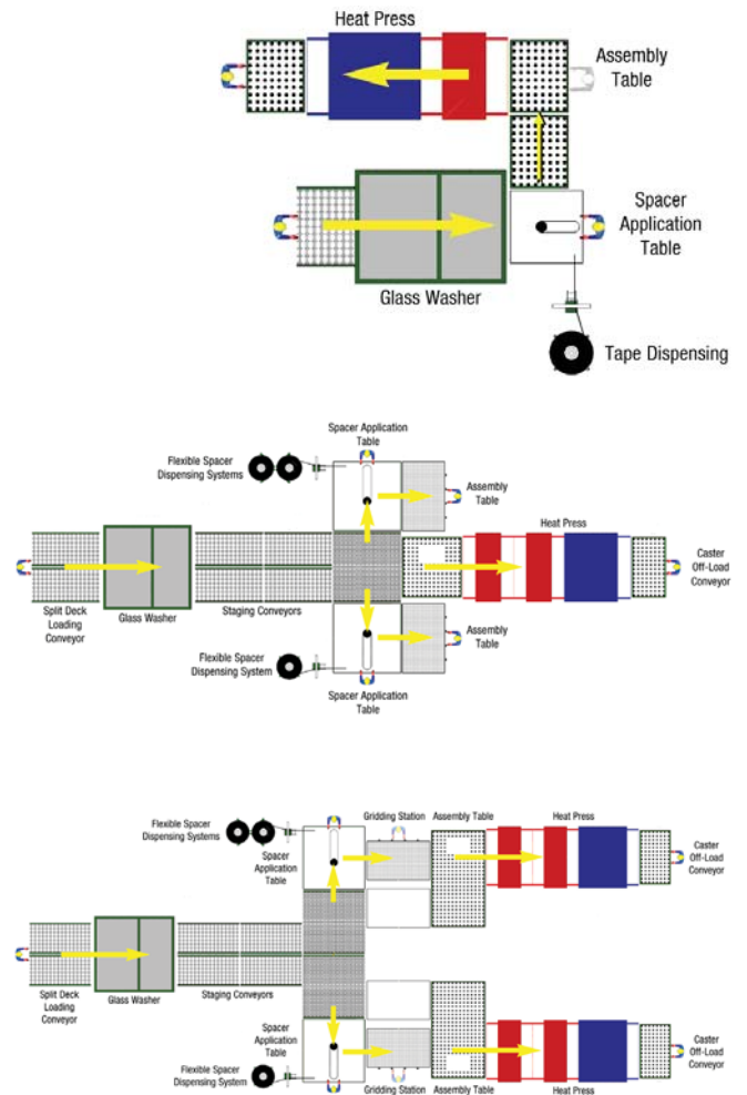
Sample Line Layouts: Basic, High Production, and Fully Automated
