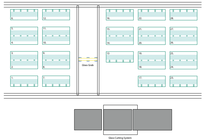
A Standard Multi-Rack Layout, Consisting of 28 Racks
